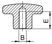
Type A Threaded blind bore 螺紋及孔未貫穿
