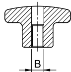
Type B Threaded through bore 螺紋及孔貫穿
